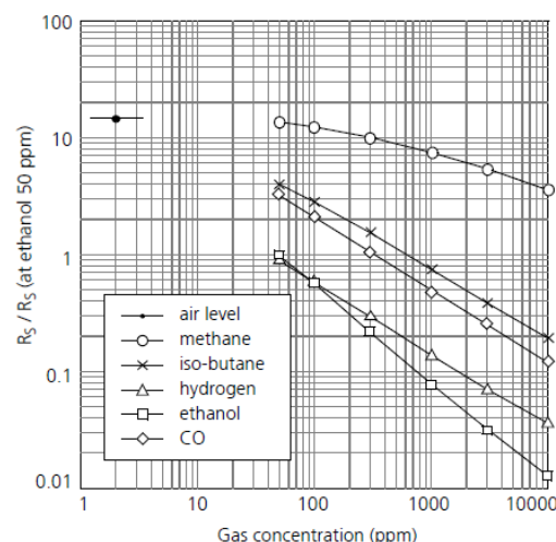
Fig3. Sensitivity characteristics
