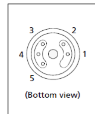
Fig 1c. Pin Layout
