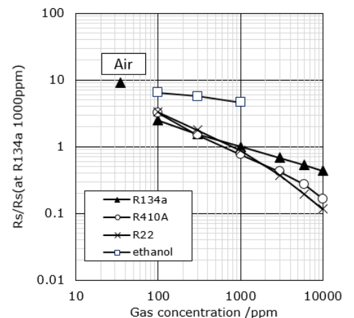
Fig 3. Sensitivity characteristics
