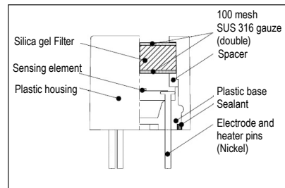
Fig 1b. Configuration
